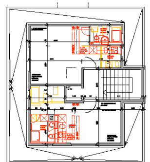
Attikageschoss
